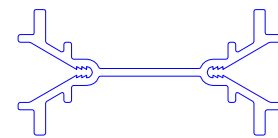
20mm Aluminium Coupling 104.210
