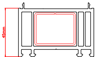
45mm frame extension 114.202 Reinforcement 113.271
