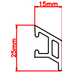
Drip Mould 109.030 End Cap 109.140
