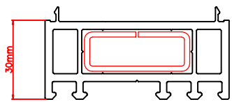
30mm frame extension 114.014 Reinforcement 113.035
