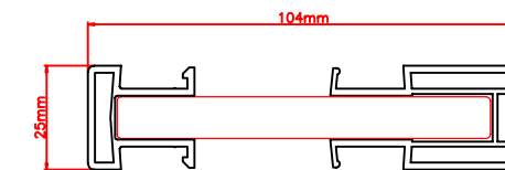
Coupling Covers 116.028 & 116.029 Reinforcement 113.121 (solid)
