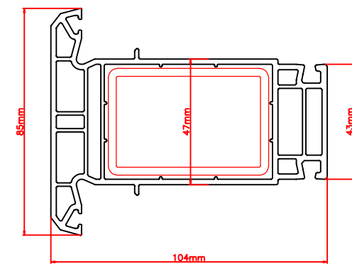
Coupling Profile 116.202 Steel Reinforcement 113.011
