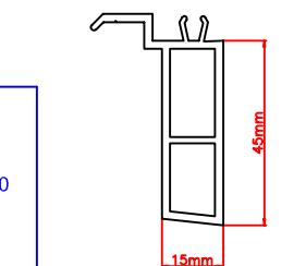
cill frame extension 110.046
