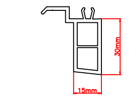
cill frame extension 110.047
