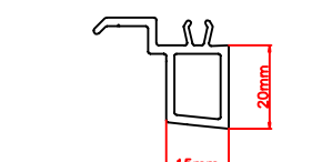
cill frame extension 110.048
