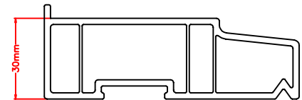
95mm stub cill extension 110.074 reinforcement 113.377 (end cap 109.074)
