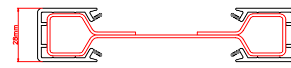
Dog Bone Coupling 113.112 Cover 116.012
