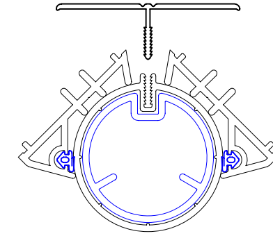
Bay Pole Cover 116.047 Aluminium Bay Pole 104.157 Bay Pole Shoe 116.049 Gasket 112.003 Cover Piece 116.048 Adjustment Nut 141.437
