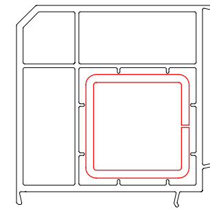
90° Corner Post 116.200 Steel Reinforcement 113.128 Aluminium Reinforcement 115.014 Adjustment Nut 141.444
