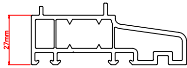
85mm stub cill extension 110.060 reinforcement 113.020 (end cap 109.368)
