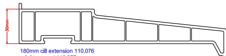
180mm cill extension 110.076 reinforcement 113.377 (end cap 109.090)
