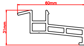
32.5mm cill frame extension 110.028
